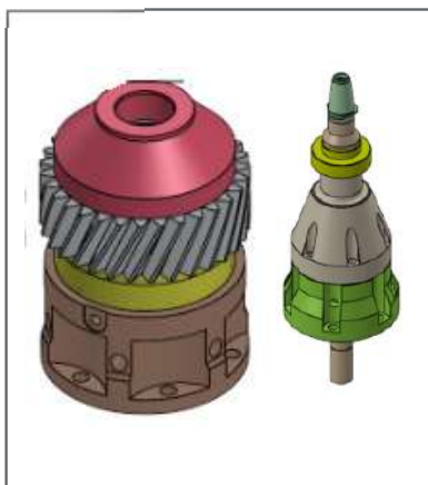
HOBGING FIXTURE
