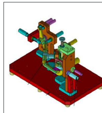
RECEIVER GAUGE OF PEDAL BRAKE
