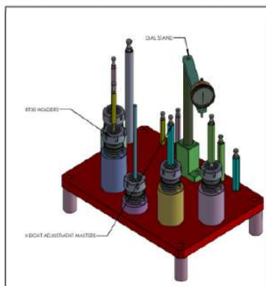
TOOL PRESETTER
