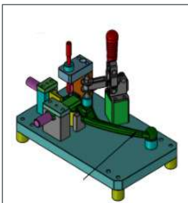
PROFILE & RECEIVER GAUGES OF LEVER
